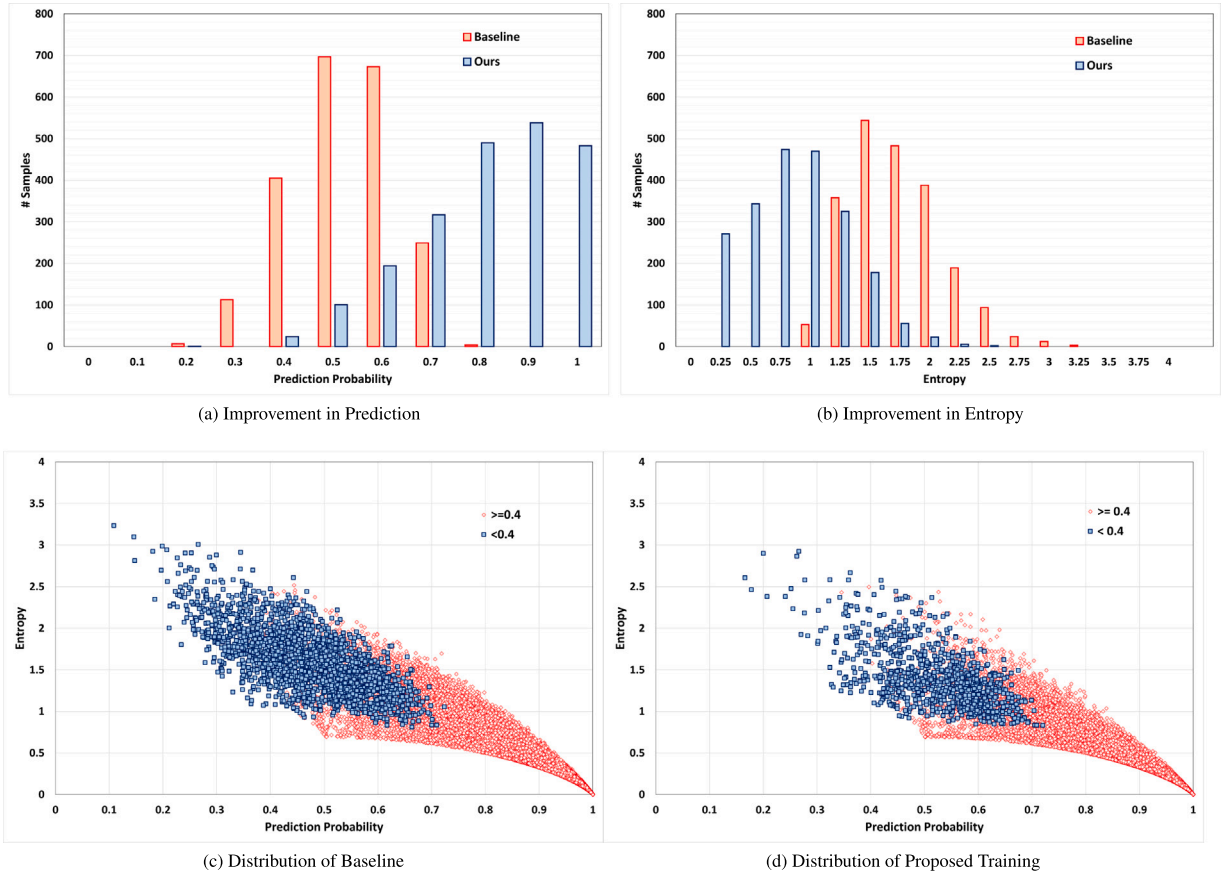
Fig. 8. Improvement experienced on the selected hard samples before and after applying data augmentation.
