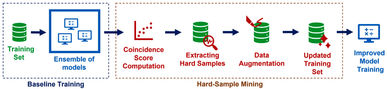
Fig. 4. Overall Training Pipeline. An ensemble is created during the baseline training; the dataset is updated using the hard samples mined using the coincidence score.
