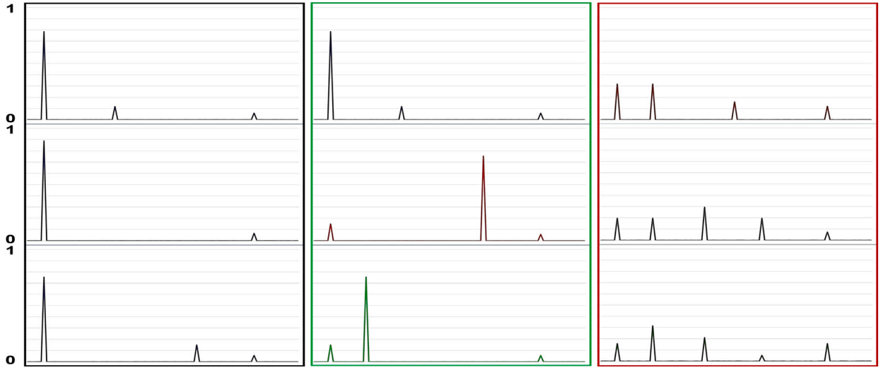
Fig. 2. Behaviour of three different models (rows) in a deep ensemble (the x-axis corresponds to the class index and the y-axis corresponds to the likelihood obtained by individual models in the ensemble). Left column: all three models predict the same class; middle column: all models predict different classes; and right column: models give low likelihood to all classes.
