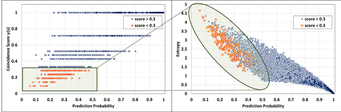
Fig. 3. Coincidence score vs. Prediction probability of samples (left plot). The relation between coincidence score and entropy is highlighted - a low coincidence score relates to high entropy.
