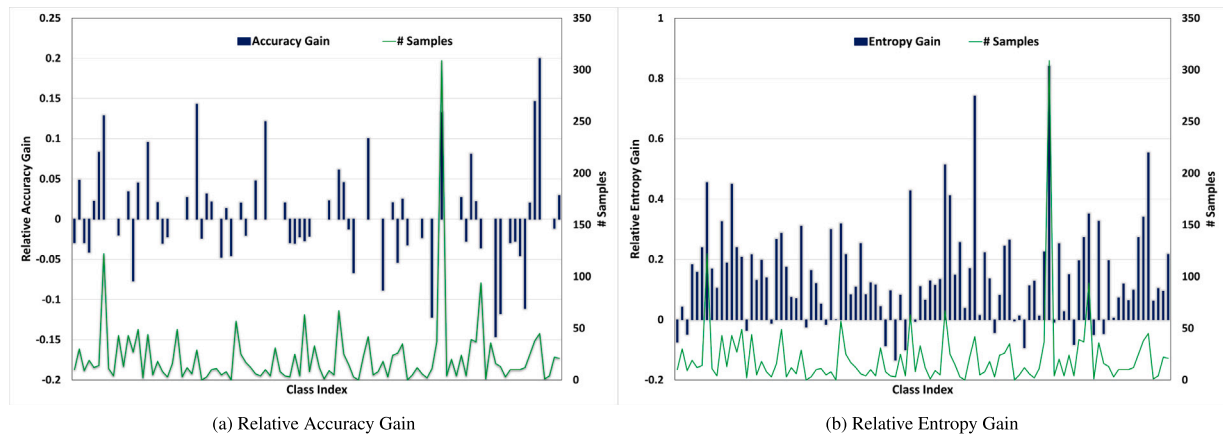
Fig. 6. Relative Gain in Performance for Food-1K(100) trained on ResNet-50.
